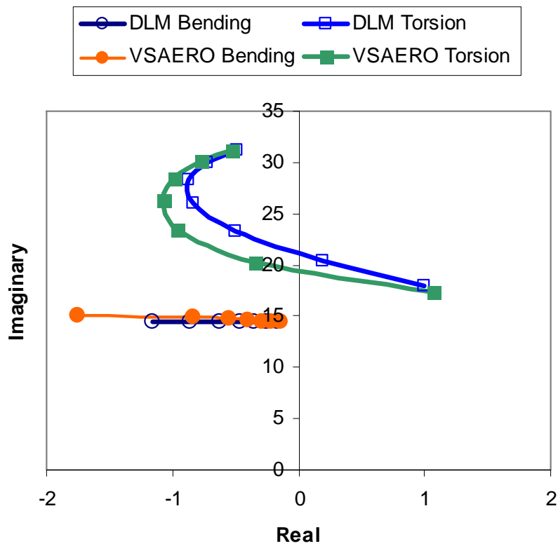
Flutter Locus of Goland and Luke Wing.
